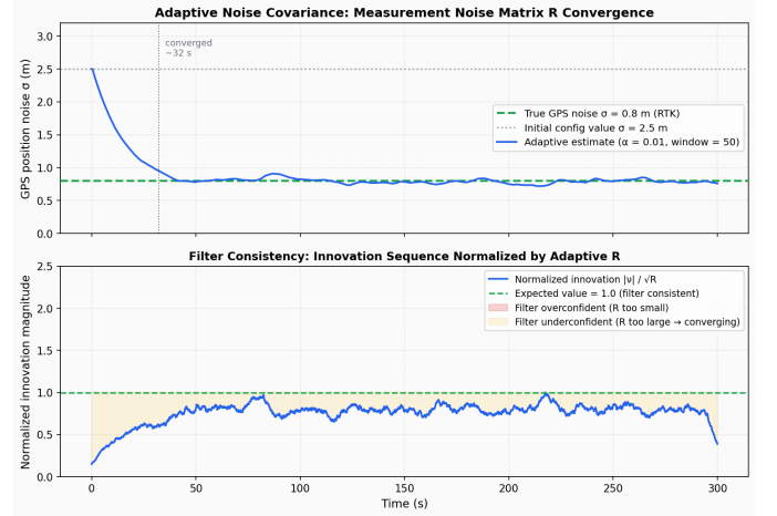
Fig. 3. Adaptive noise convergence. Starting at \sigma = 2.5 m, the estimate converges to the true GPS noise ( \sigma = 0.8 m) within 32 s. The normalized innovation sequence approaches 1.0, indicating a consistent filter.
