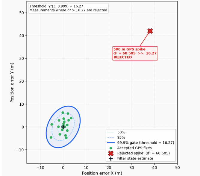
Mahalanobis Outlier Gate: Chi-squared Rejection at 3 DOF, 99.9th Percentile
