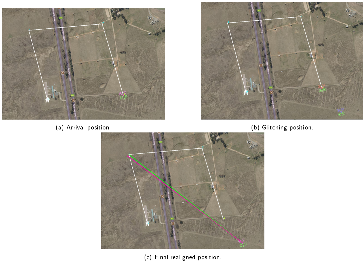
Figure 5: Final map view of the progressive GPS spoofing.
