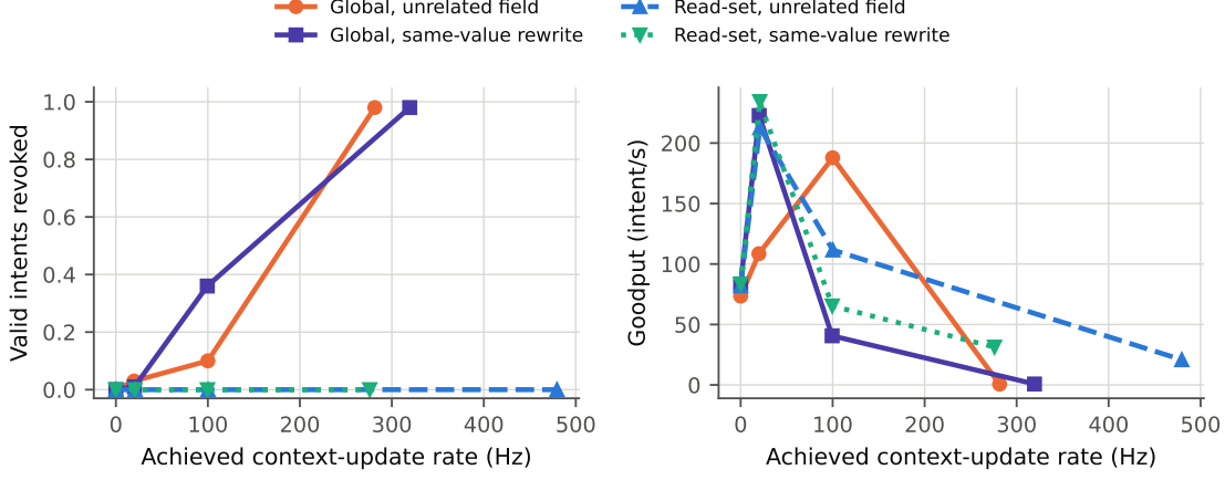
Single-host campaign: false revocations (left) and goodput of valid intents (right) against the achieved update rate. Read-set versions revoke none.
