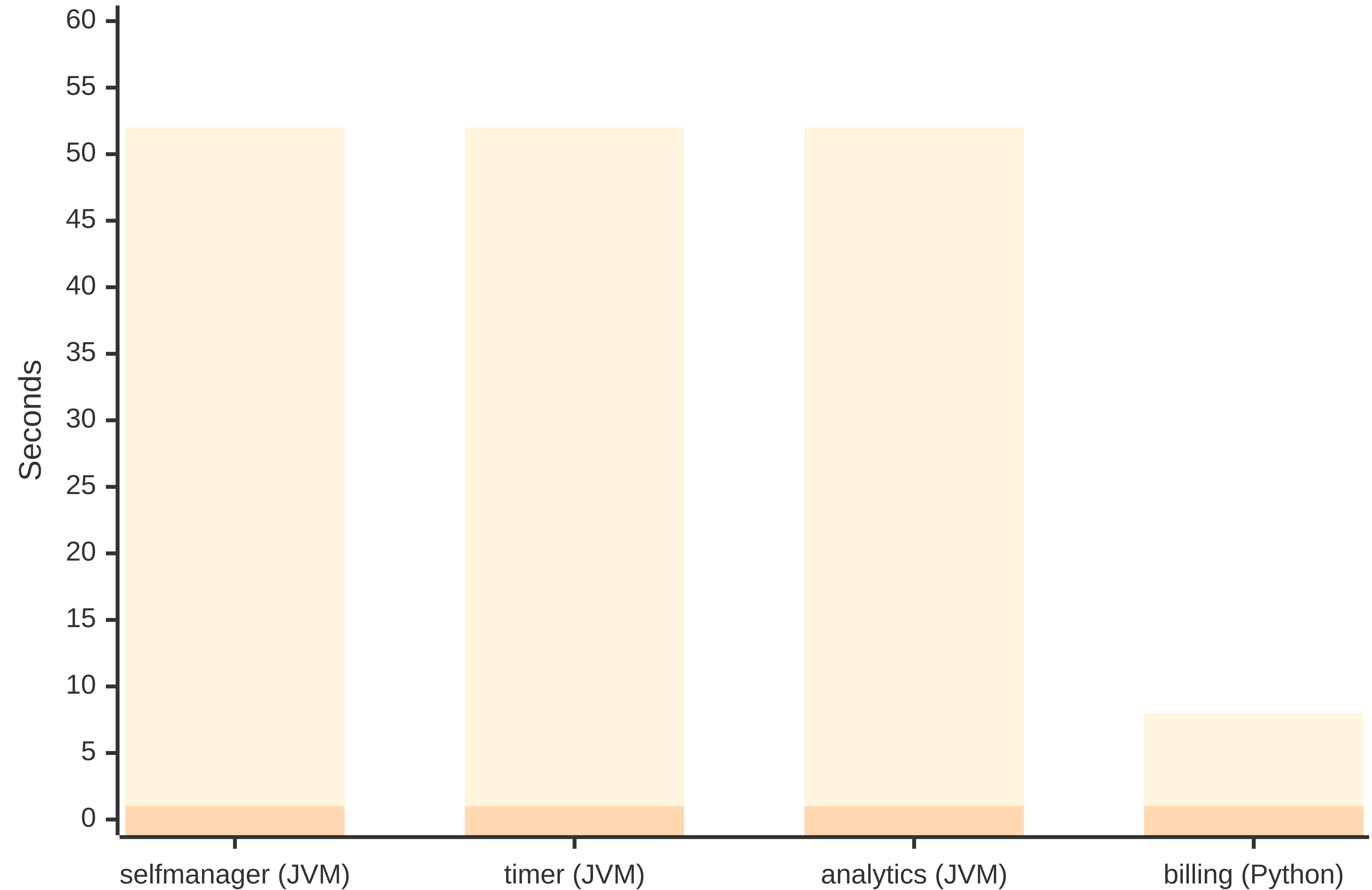
Cold Start vs Warm Response Time by Service (seconds)
