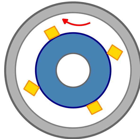
FREEWHEELING (Overrunning)
