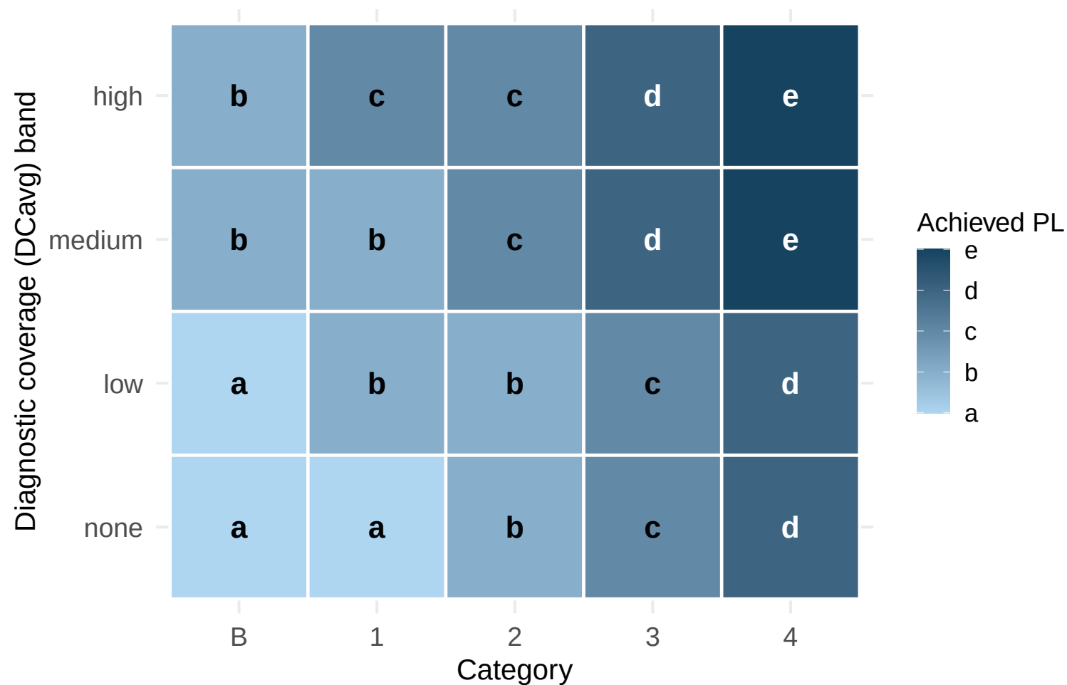
Illustrative Achieved PL by Category and DCavg (MTTFd = "high")
