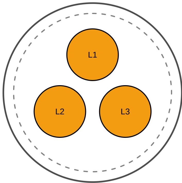
TECK90 (interlocked armor + PVC jacket)
