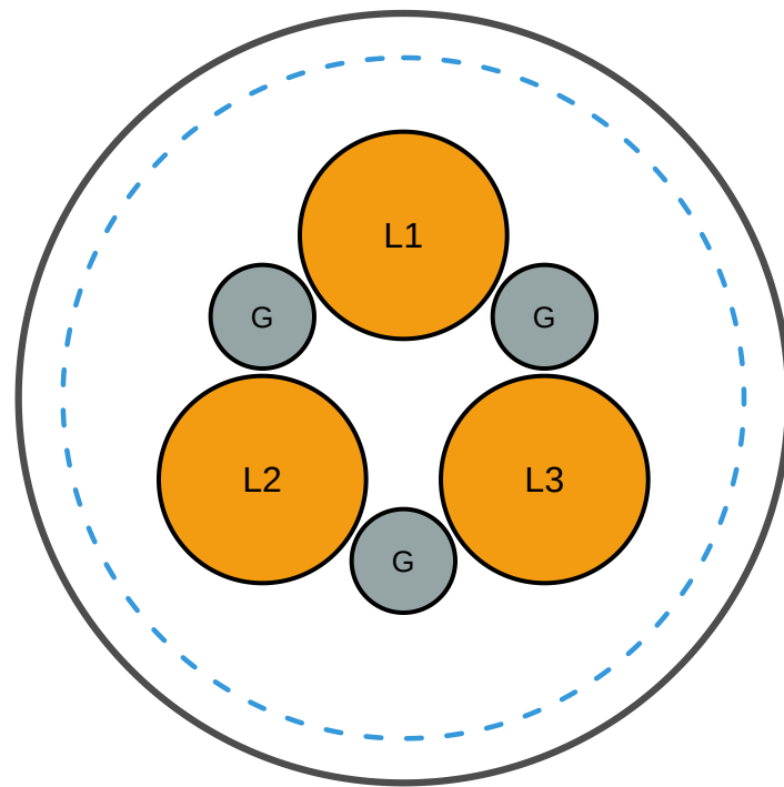
VFD Cable (shielded, symmetrical ground conductors)
