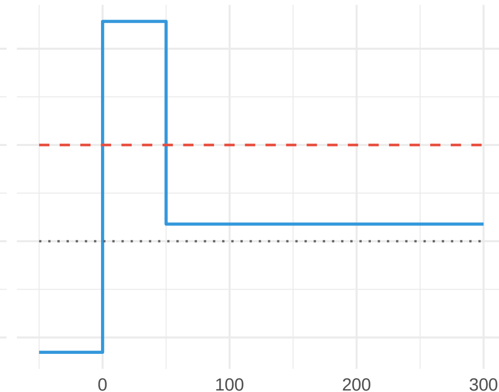
Fault: all 14 valves + 4 contactors
