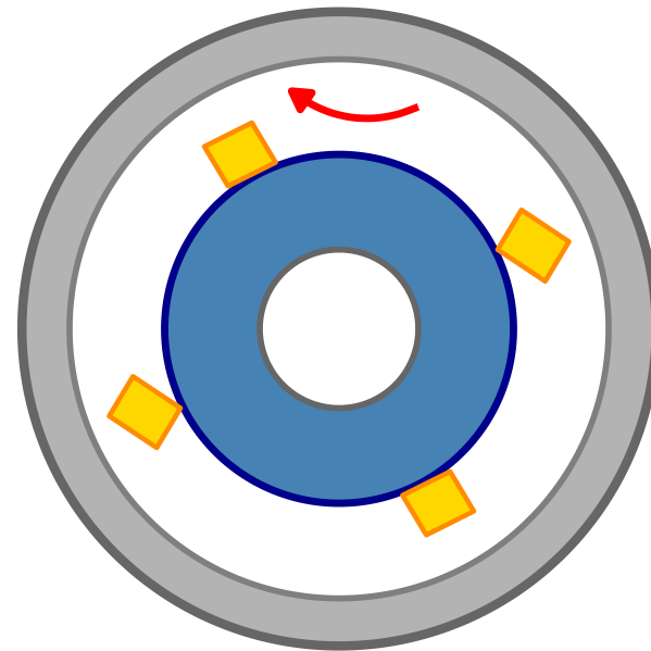
FREEWHEELING (Overrunning)
