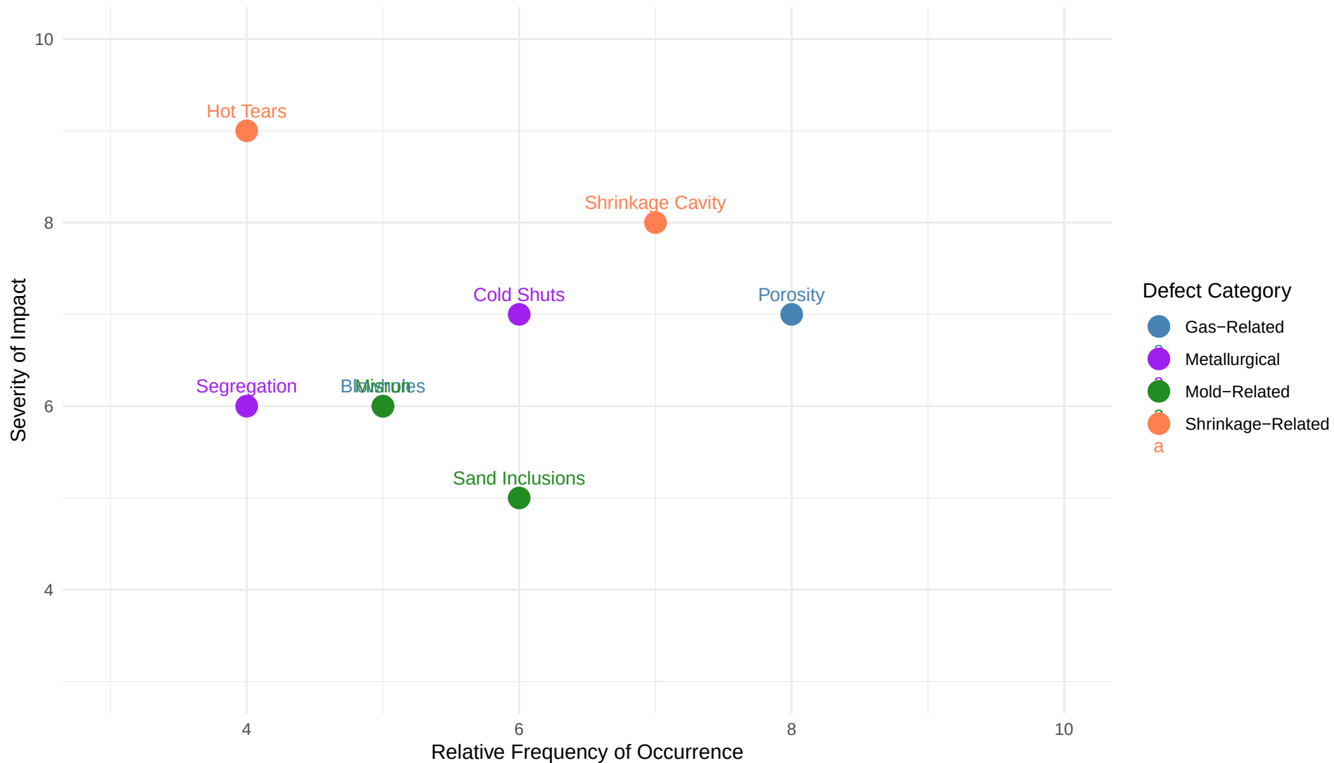
Casting Defects: Severity vs. Frequency
