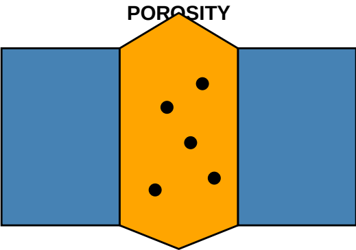
Gas pockets trapped in weld
