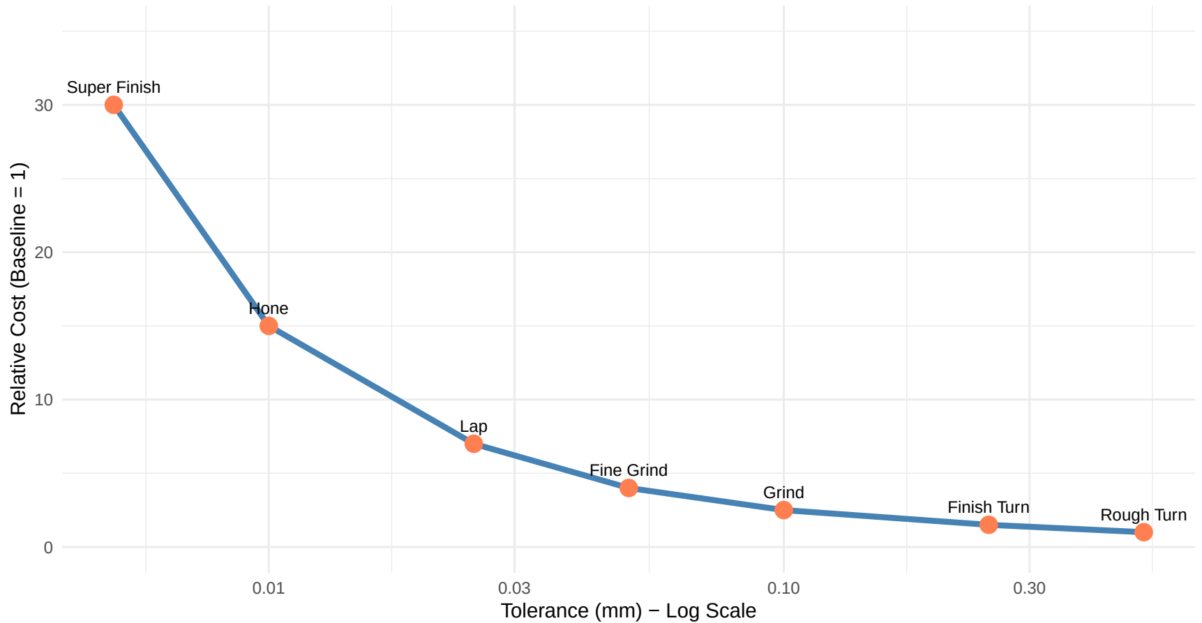
Tolerance vs. Machining Cost
