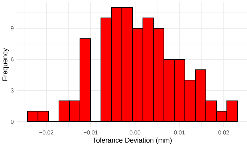
Distribution of Machining Tolerances
