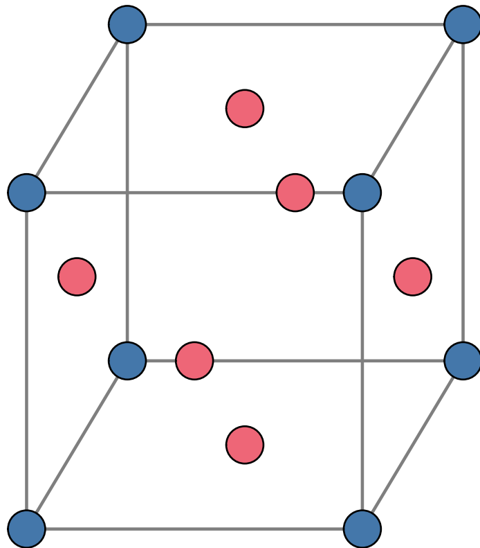
FCC (austenite)
