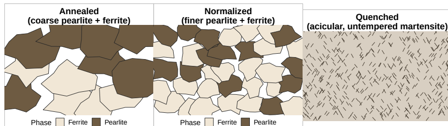
Figure 20.6: Schematic diagram (not an actual photomicrograph) comparing three heat-treated conditions of the same steel at the same scale: annealed (coarse pearlite + ferrite), normalized (finer pearlite + ferrite), and quenched (acicular, untempered martensite).
