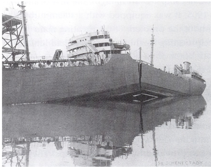
Figure 20.4: The SS Schenectady , a Liberty-ship-type T2 tanker, moored at the dock in Portland, Oregon, after her welded hull fractured almost completely in two on 16 January 1943 — a dramatic, non-fatal example of exactly the brittle fracture this section describes. (U.S. Government Printing Office, 1947; public domain, via Wikimedia Commons.)
