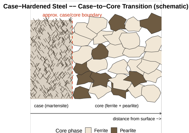
Figure 20.5: Schematic diagram (not an actual photomicrograph) of a case-hardened cross-section: a dense, acicular (needle-like) martensite/tempered-martensite case near the surface, transitioning to coarser ferrite+pearlite grains in the core. The boundary is drawn sharp for clarity; a real transition is more gradual.
