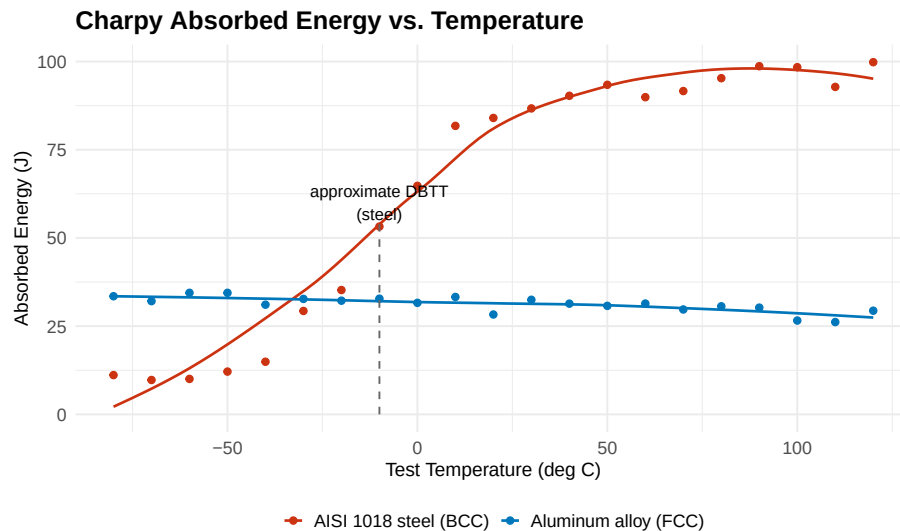
Figure 20.3: Representative Charpy absorbed energy vs. temperature curves: a BCC steel shows a sharp ductile-to-brittle transition; an FCC aluminum alloy stays comparatively flat across the same temperature range (schematic, typical shapes only).
