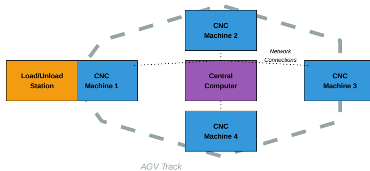
Figure 6.9: Flexible Manufacturing System Components
