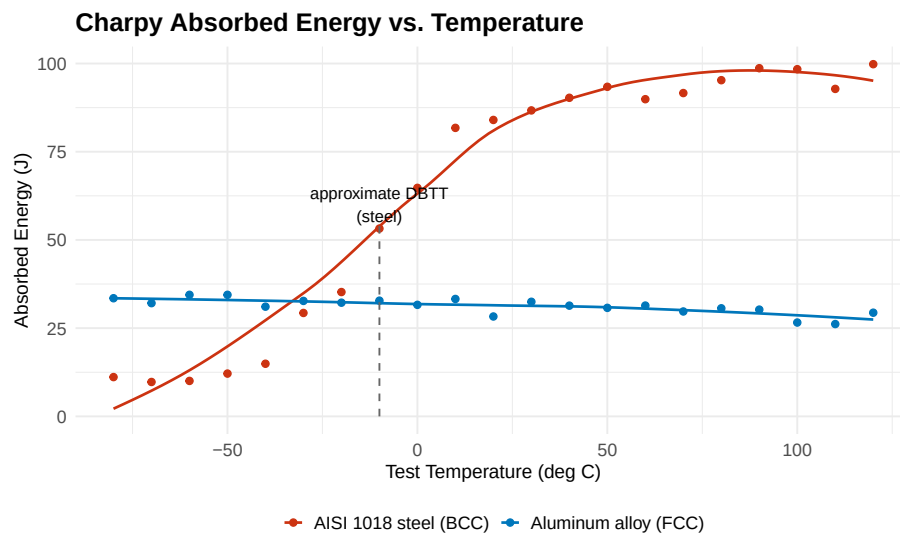
Figure 20.3: Representative Charpy absorbed energy vs. temperature curves: a BCC steel shows a sharp ductile-to-brittle transition; an FCC aluminum alloy stays comparatively flat across the same temperature range (schematic, typical shapes only).
