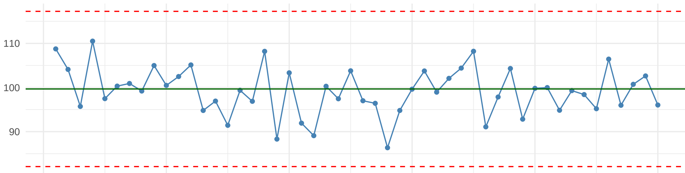
Poor MSA (%GRR = 93%)
