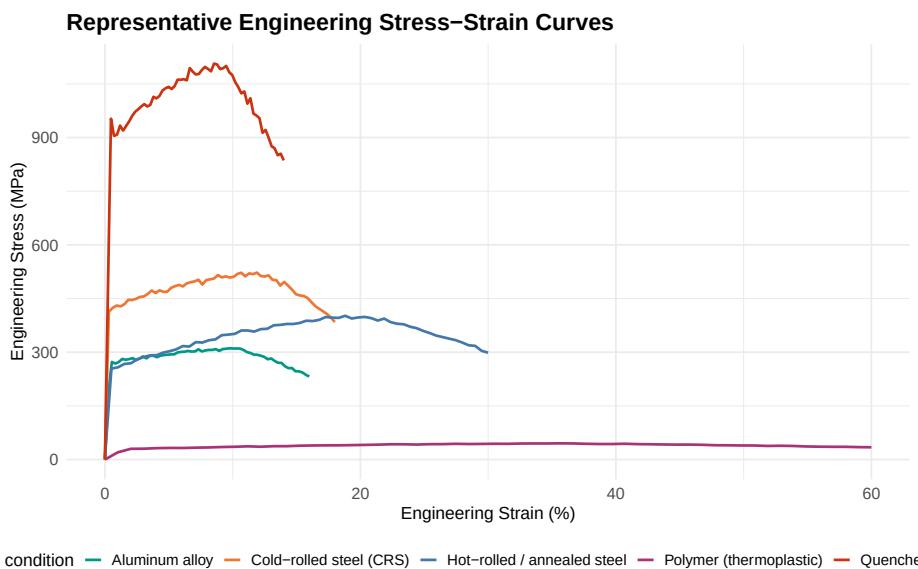
Figure 20.1: Representative engineering stress-strain curves for several material conditions (schematic, typical shapes only – actual curves depend on exact grade, condition, and specimen). CRS and quenched-and-tempered steel show higher strength but lower ductility than HRS/annealed steel; aluminum shows no sharp yield point; the polymer shows a much lower modulus and a very different curve shape.
