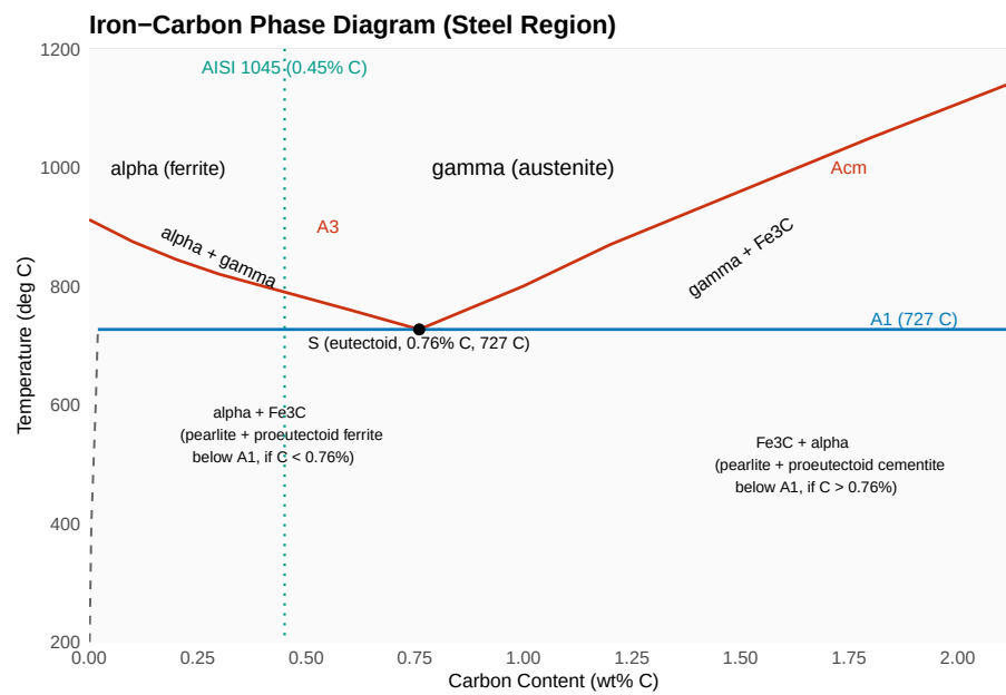
Figure 19.5: The iron-carbon phase diagram, steel region only (0 to 2.14 wt% C). A3 and Acm curves are smoothed approximations for teaching purposes; consult a reference diagram (e.g. Callister) for precise values.
