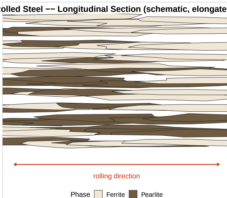
Figure 19.4: Schematic diagram (not an actual photomicrograph) of cold-rolled 1018 steel, longitudinal section: grains visibly stretched and lined up parallel to the rolling direction. A transverse section of the same bar would look nearly as equiaxed as HRS – see Section 19.4.2.
