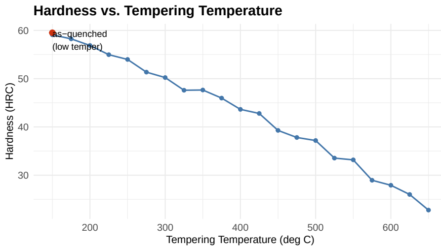
Figure 19.6: Typical hardness of a quenched medium-carbon steel as a function of tempering temperature (simulated, illustrative trend only – actual curves vary by alloy and carbon content).
