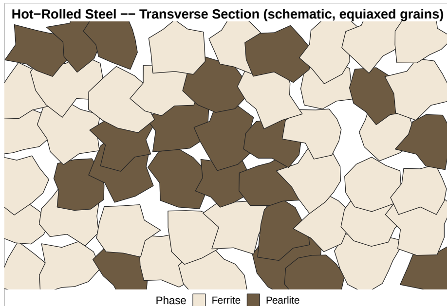
Figure 19.3: Schematic diagram (not an actual photomicrograph) of hot-rolled 1018 steel: equiaxed grains, similar in every direction, regardless of which way the section is cut.
