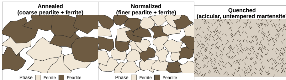
Figure 20.4: Schematic diagram (not an actual photomicrograph) comparing three heat-treated conditions of the same steel at the same scale: annealed (coarse pearlite + ferrite), normalized (finer pearlite + ferrite), and quenched (acicular, untempered martensite).
