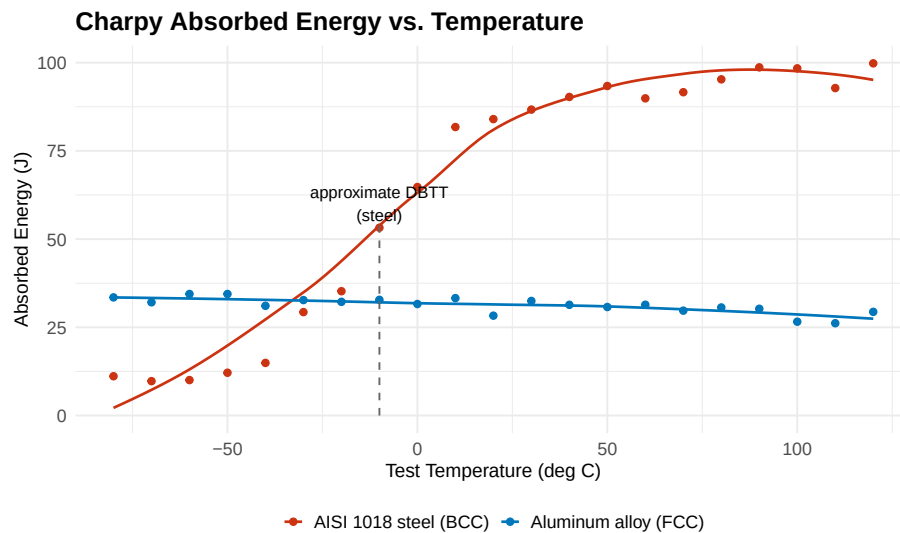
Figure 20.2: Representative Charpy absorbed energy vs. temperature curves: a BCC steel shows a sharp ductile-to-brittle transition; an FCC aluminum alloy stays comparatively flat across the same temperature range (schematic, typical shapes only).
