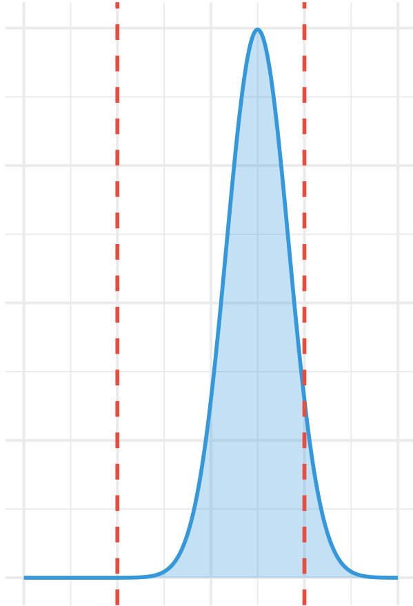
Shifted ( C_p=2 , C_{pk}=1 )
