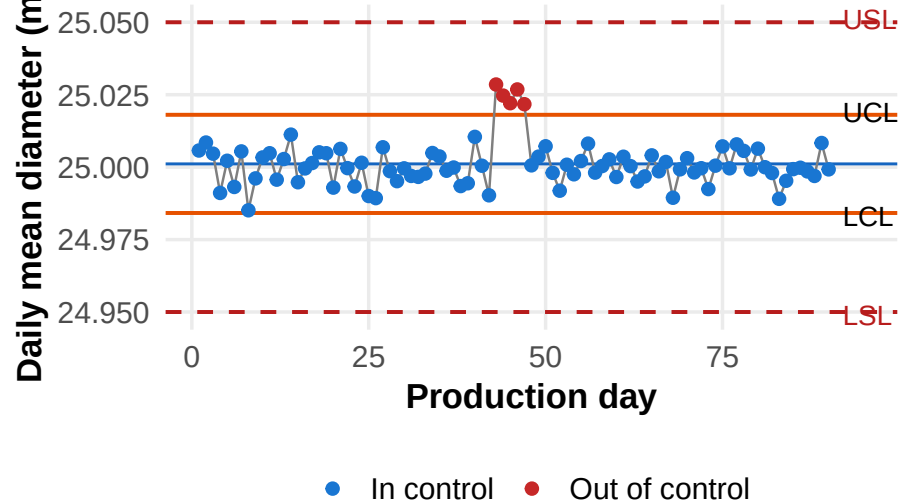
Figure 18.3: Simulated X-bar control chart for daily mean diameter over 90 production days. A special-cause event (bad bar stock) is visible around days 43–47 — the same event you will find in the Week 2 lab dataset.
