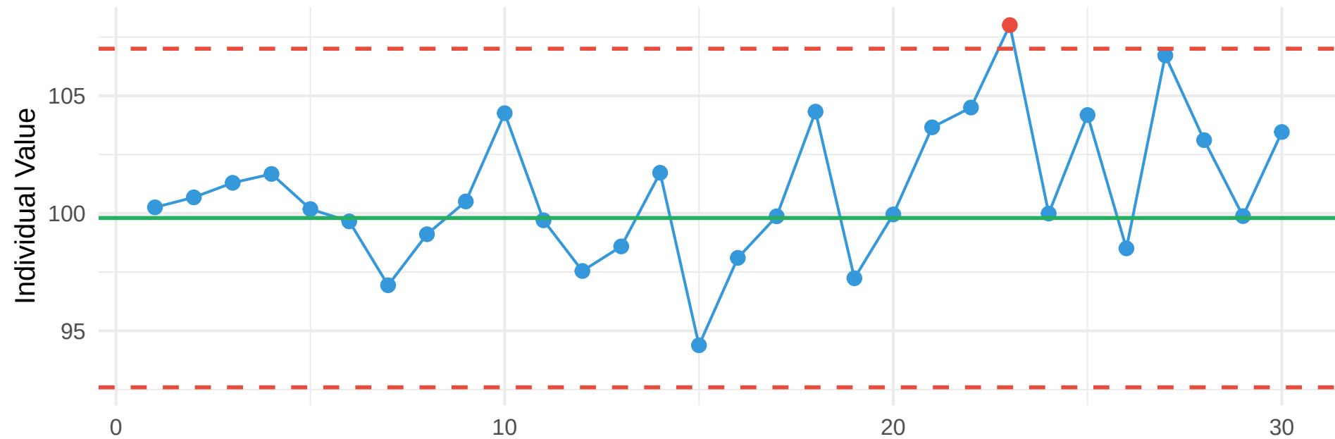
Individual (I) Chart
