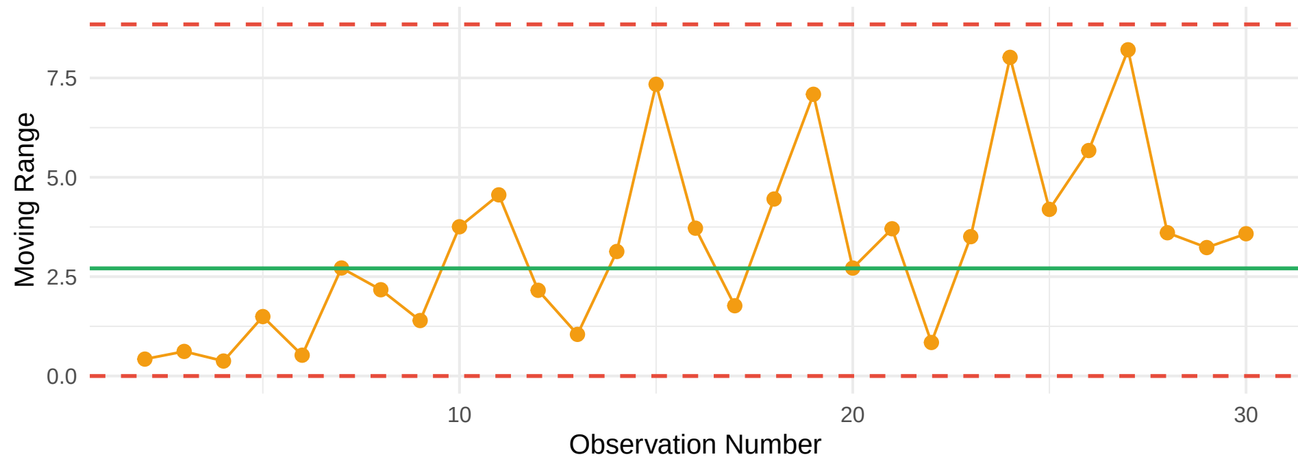
Moving Range (MR) Chart
