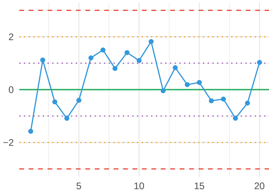
Rule 3: 4 of 5 in Zone B
