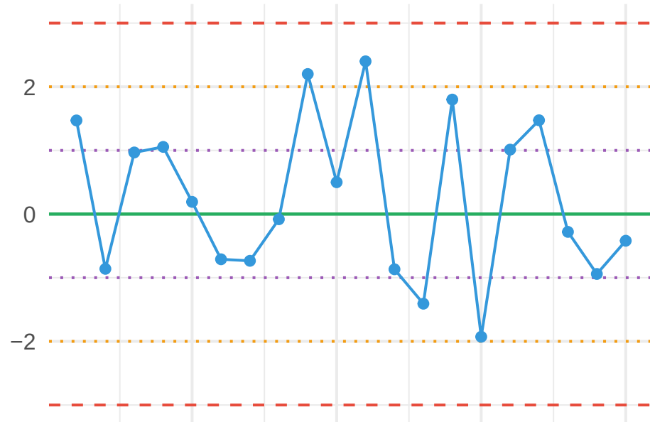
Rule 2: 2 of 3 in Zone A
