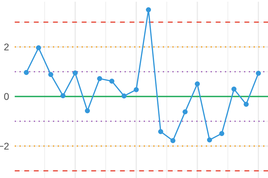
Rule 1: Beyond Limit
