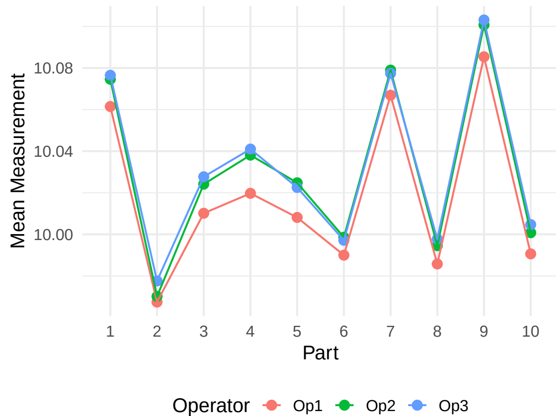
Part × Operator Interaction
