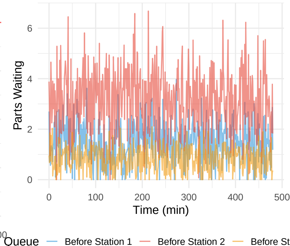
Queue Lengths
