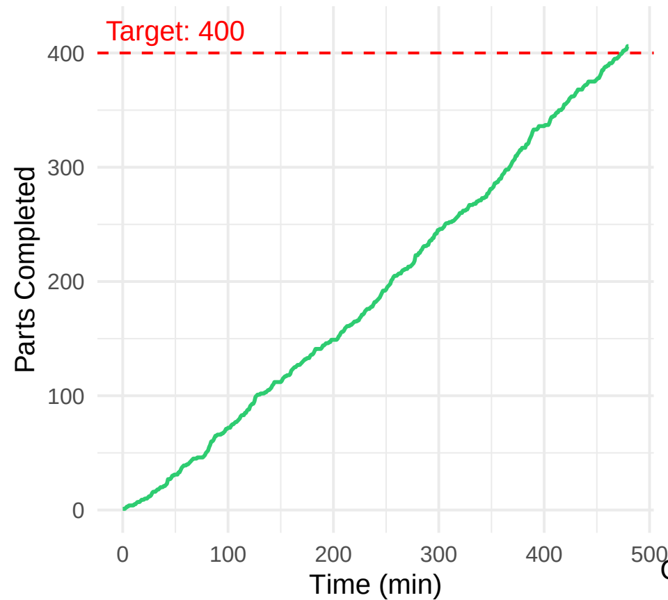
Cumulative Throughput
