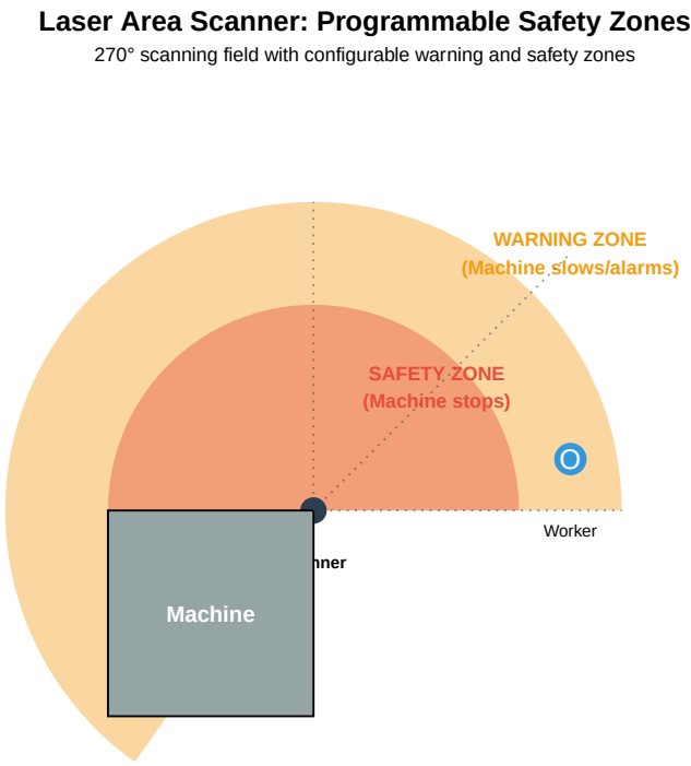
Figure 9.7: Laser Area Scanner Zones
