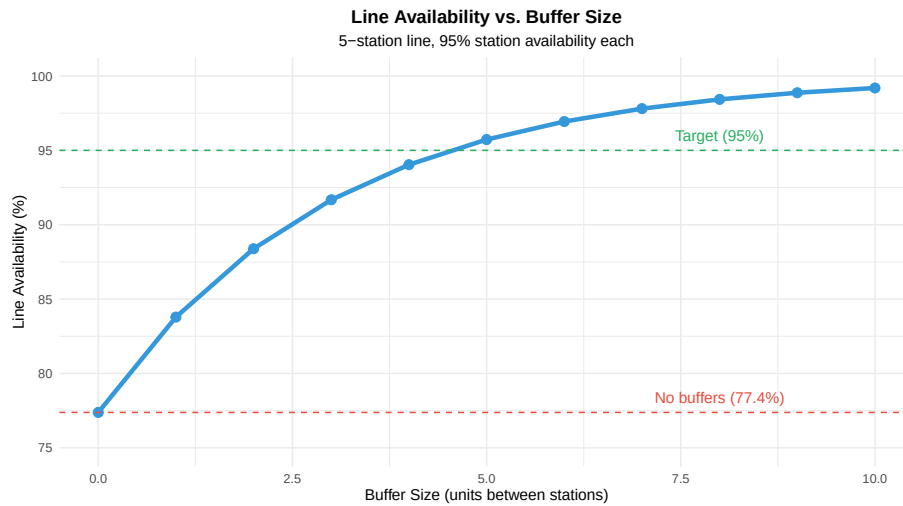
Figure 3.7: Effect of Buffers on Line Availability
