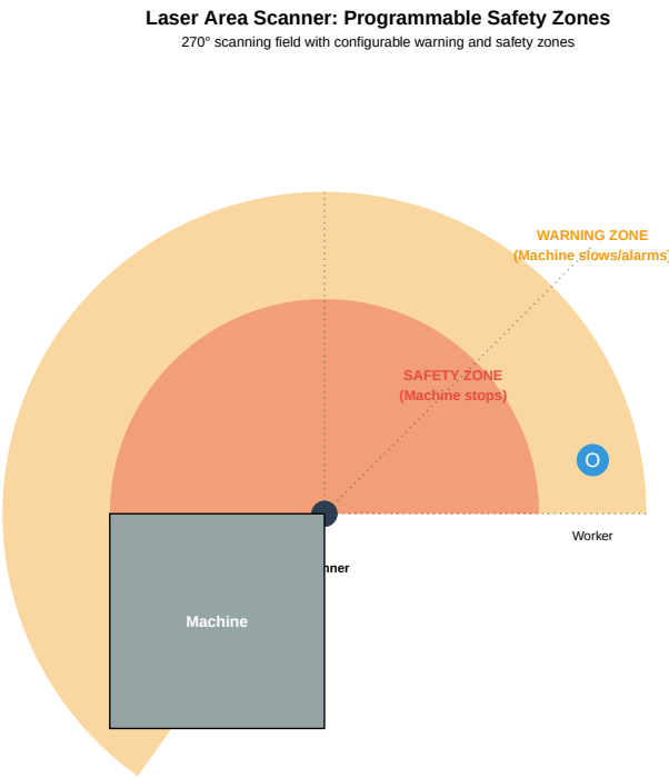
Figure 6.7: Laser Area Scanner Zones
