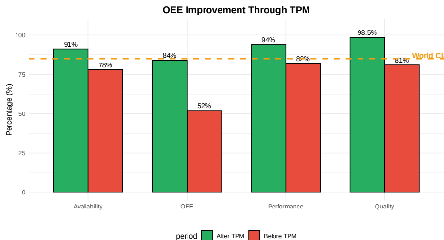
Figure 12.14: OEE Improvement: Before and After TPM
