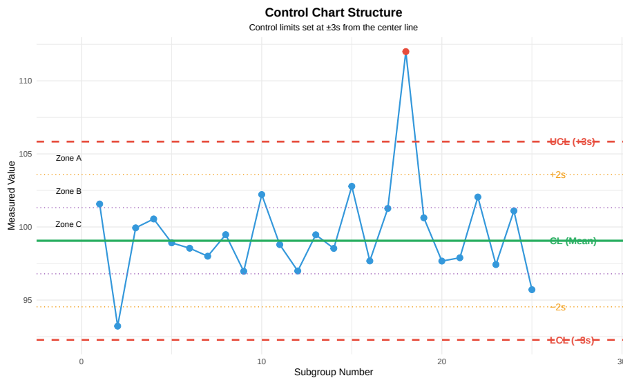
Figure 10.6: Anatomy of a Control Chart
