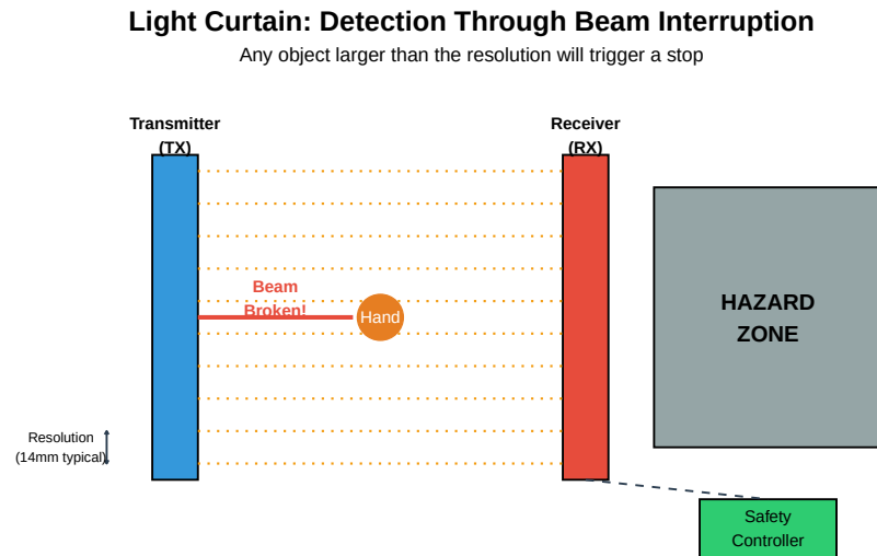
Figure 6.6: Light Curtain Operating Principle
