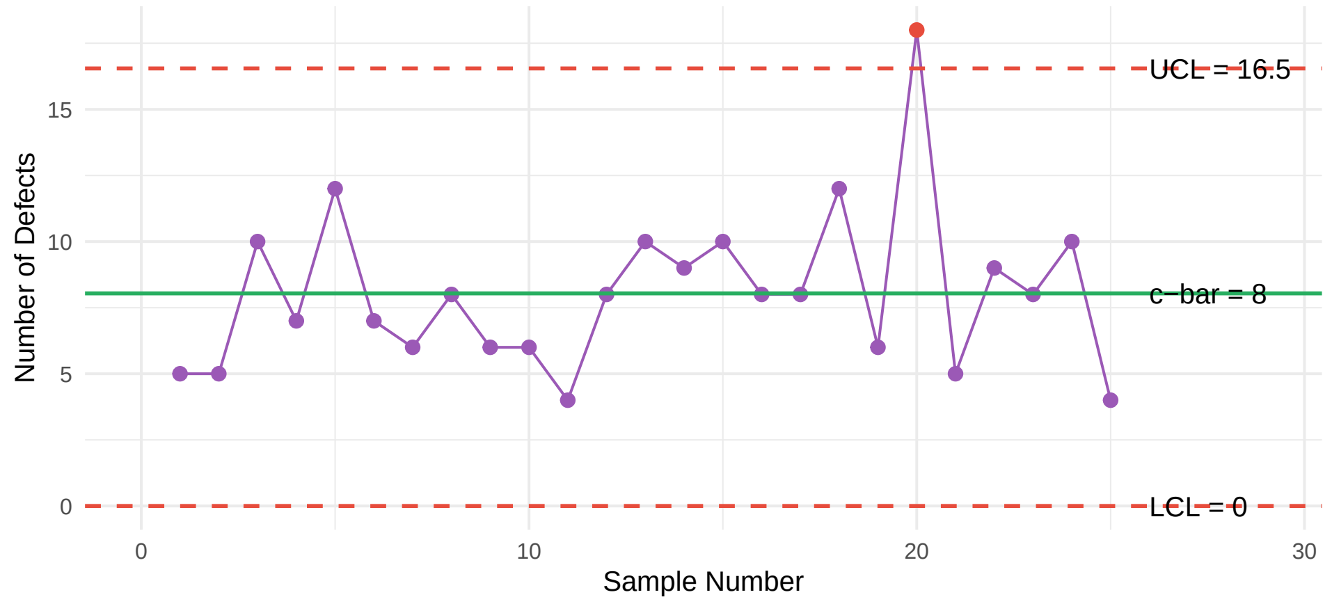
c Chart: Defects per Car Body
