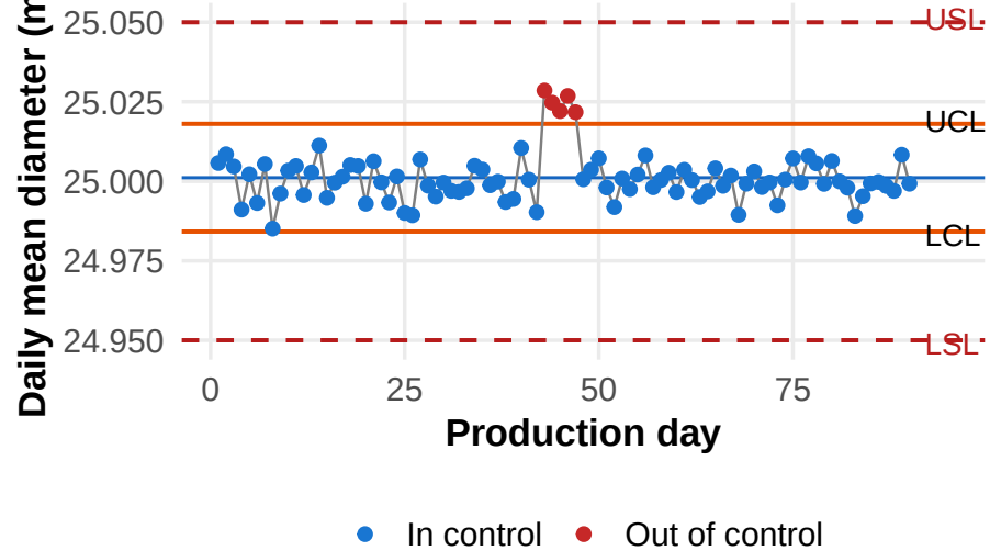
Figure 13.3: Simulated X-bar control chart for daily mean diameter over 90 production days. A special-cause event (bad bar stock) is visible around days 43–47 — the same event you will find in the Week 2 lab dataset.
