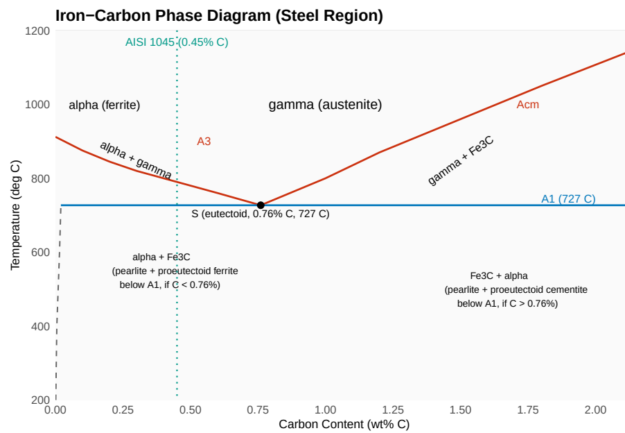
Figure 19.5: The iron-carbon phase diagram, steel region only (0 to 2.14 wt% C). A 3 and A cm curves are smoothed approximations for teaching purposes; consult a reference diagram (e.g. Callister) for precise values.
