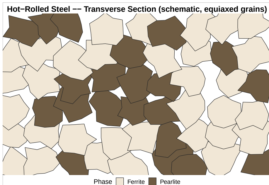
Figure 19.3: Schematic diagram (not an actual photomicrograph) of hot-rolled 1018 steel: equiaxed grains, similar in every direction, regardless of which way the section is cut.
