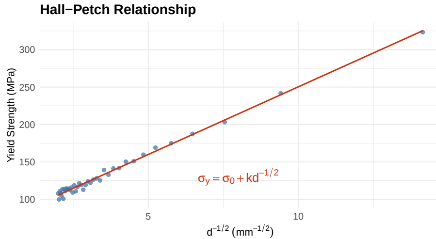
Figure 19.2: The Hall-Petch relationship: yield strength rises as grain size decreases, and rises steeply once grains become very fine (data simulated for a low-carbon steel, \sigma_0 = 70 MPa, k = 18 MPa*mm 0.5 ).
