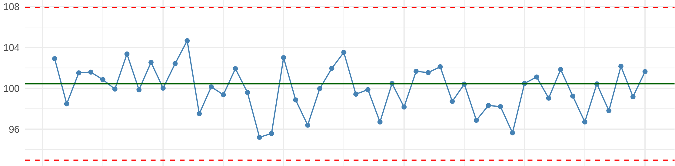
Good MSA (%GRR = 10%)
