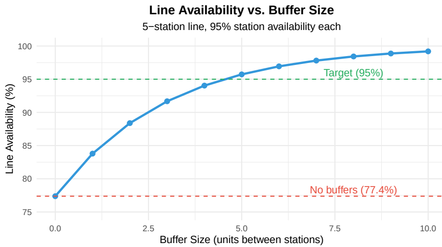
Figure 6.7: Effect of Buffers on Line Availability
