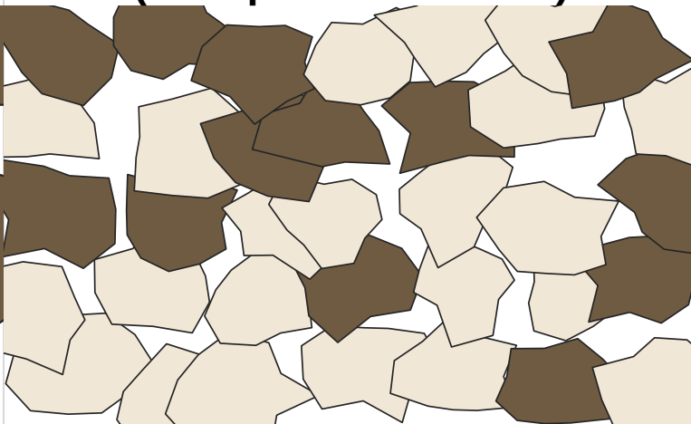
Normalized (finer pearlite + ferrite)
