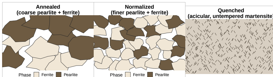
Figure 20.8: Schematic diagram (not an actual photomicrograph) comparing three heat-treated conditions of the same steel at the same scale: annealed (coarse pearlite + ferrite), normalized (finer pearlite + ferrite), and quenched (acicular, untempered martensite).
