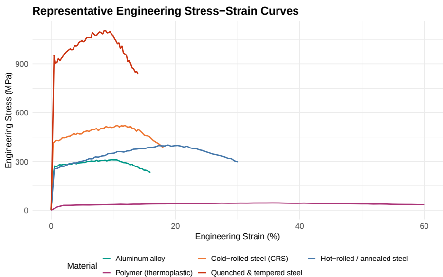
Figure 20.1: Representative engineering stress-strain curves for several material conditions (schematic, typical shapes only – actual curves depend on exact grade, condition, and specimen). CRS and quenched-and-tempered steel show higher strength but lower ductility than HRS/annealed steel; aluminum shows no sharp yield point; the polymer shows a much lower modulus and a very different curve shape.
