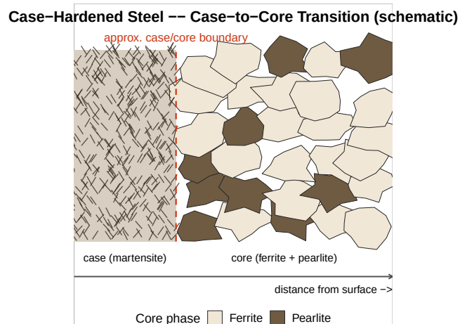
Figure 20.7: Schematic diagram (not an actual photomicrograph) of a case-hardened cross-section: a dense, acicular (needle-like) martensite/tempered-martensite case near the surface, transitioning to coarser ferrite+pearlite grains in the core. The boundary is drawn sharp for clarity; a real transition is more gradual.
