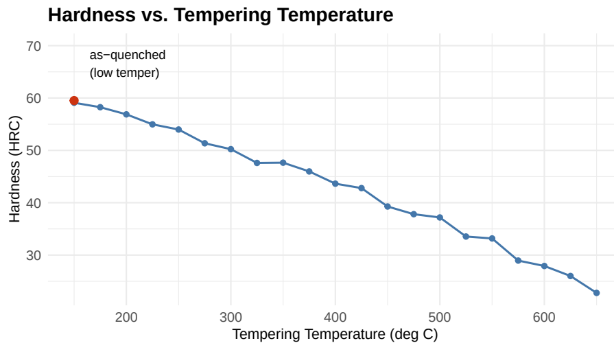
Figure 19.7: Typical hardness of a quenched medium-carbon steel as a function of tempering temperature (simulated, illustrative trend only – actual curves vary by alloy and carbon content).
