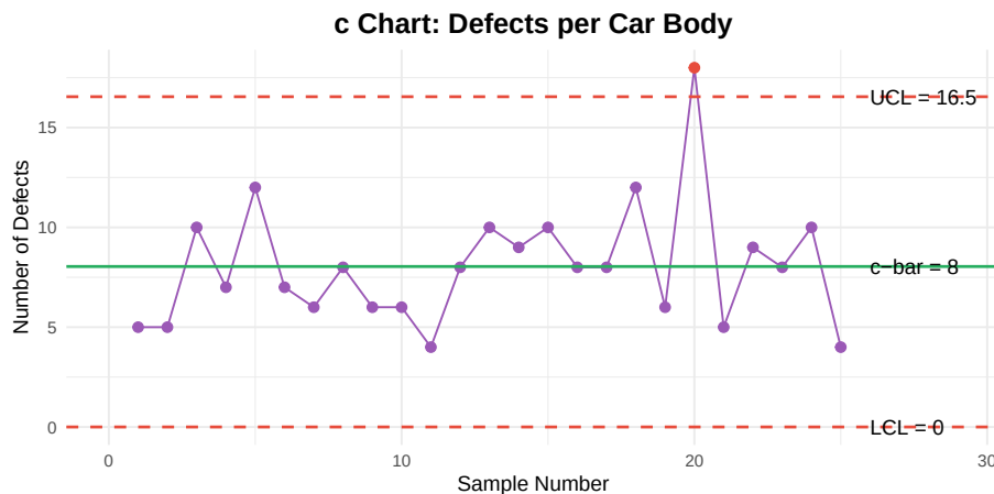
Figure 10.12: c Chart for Defects per Unit
