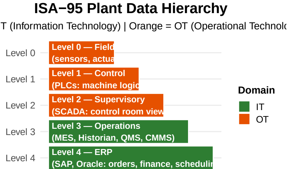
Figure 13.2: The ISA-95 data hierarchy. Levels 0–2 are Operational Technology (OT); Levels 3–4 are Information Technology (IT). Python scripts belong at Level 3 or higher — never on a PLC.
