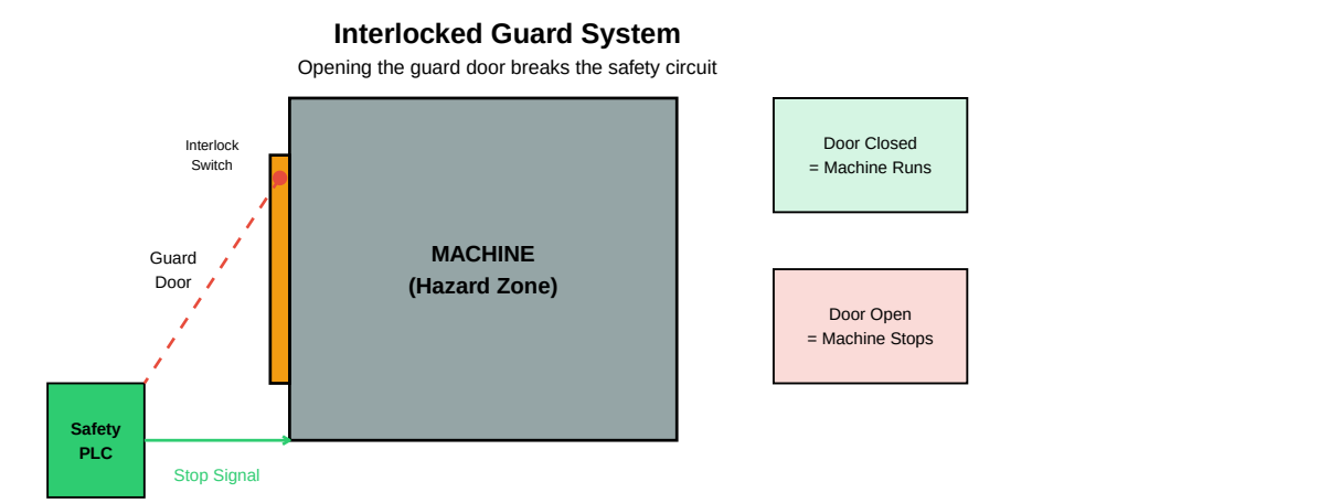
Figure 9.3: Interlocked Guard Operation Principle
