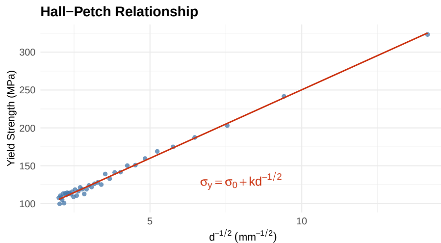
Figure 19.2: The Hall-Petch relationship: yield strength rises as grain size decreases, and rises steeply once grains become very fine (data simulated for a low-carbon steel, \sigma_0 = 70 \text{ MPa} , k = 18 \text{ MPa} \cdot \text{mm}^{0.5} ).
