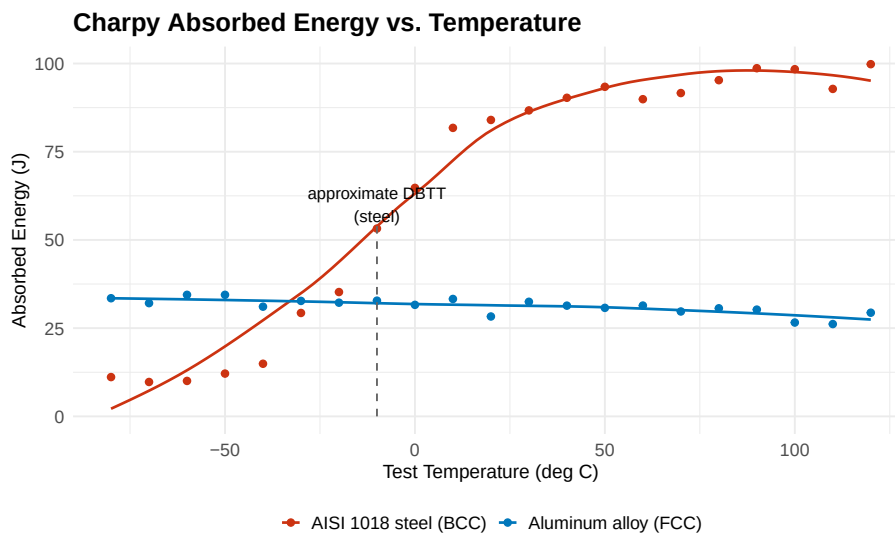
Figure 20.5: Representative Charpy absorbed energy vs. temperature curves: a BCC steel shows a sharp ductile-to-brittle transition; an FCC aluminum alloy stays comparatively flat across the same temperature range (schematic, typical shapes only).
