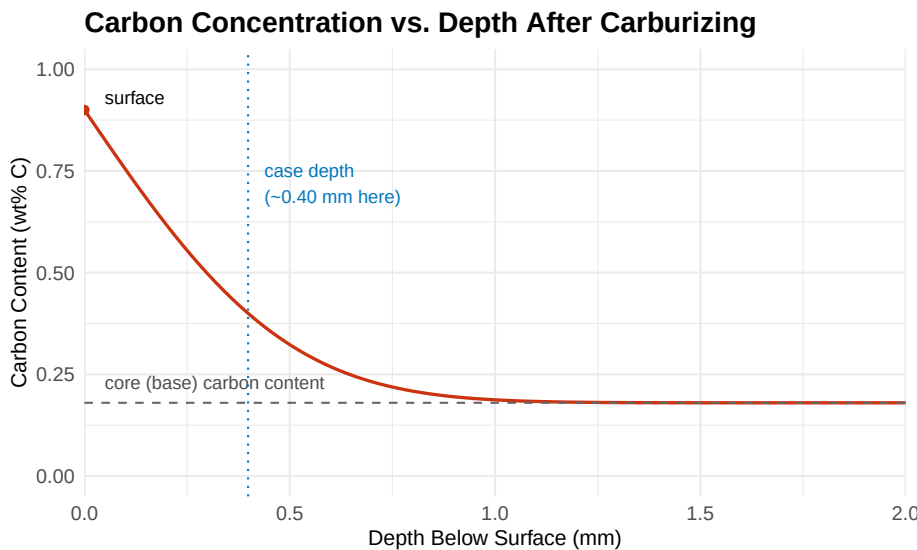
Figure 19.8: Illustrative carbon concentration profile after gas carburizing (schematic, not measured data). Carbon is highest at the surface, set by the furnace atmosphere, and falls off smoothly with depth — an error-function-shaped curve, which is the solution to Fick’s second law for this situation — down to the steel’s original core carbon content. ‘Case depth’ is conventionally defined as the depth at which carbon content falls to a chosen threshold, often 0.4% C.
