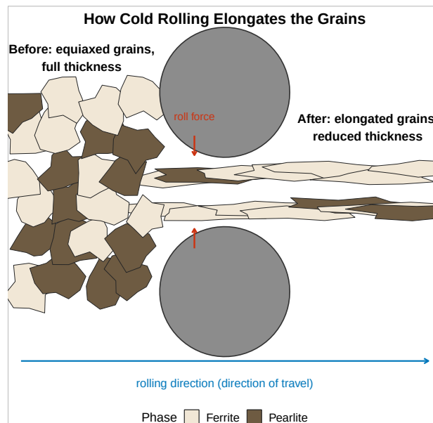
Figure 19.3: Schematic of the cold rolling mechanism (not to scale). Stock enters the roll gap at full thickness with equiaxed grains; the work rolls squeeze it under heavy compressive force; it exits thinner, with the same grains flattened in the thickness direction and stretched out in the rolling direction. This is the mechanism behind the elongated-grain micrograph in Figure 19.5.
