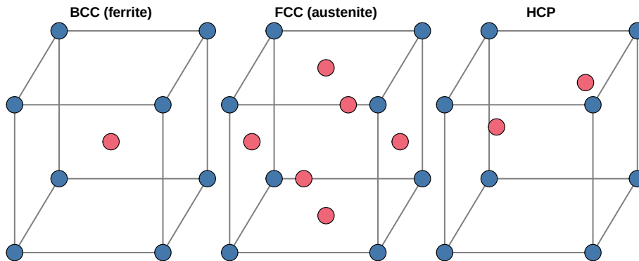
Figure 19.1: Simplified 2-D schematics of the three crystal structures that matter most for this course. Corner atoms are shared with neighbouring cells; BCC adds one body-centred atom, FCC adds one atom centred on each visible face.
