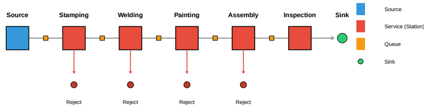
Figure 5.5: AnyLogic production line model structure
