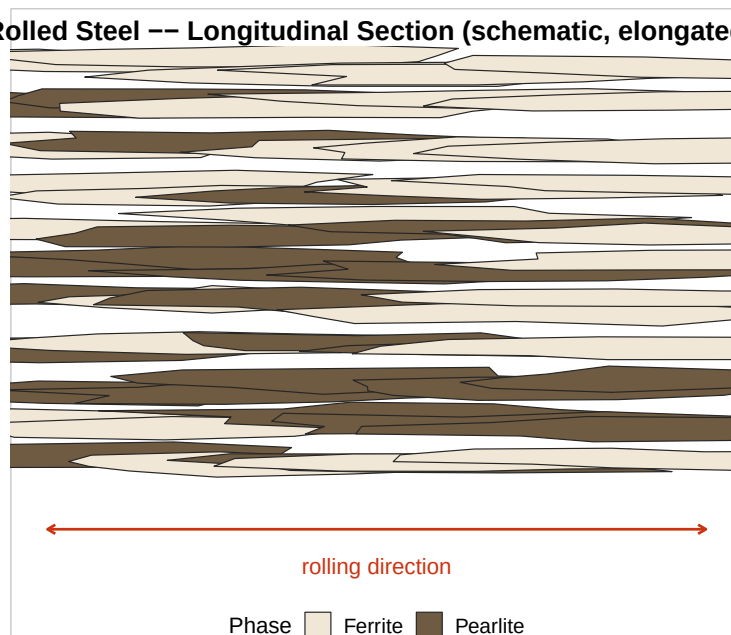
Figure 19.5: Schematic diagram (not an actual photomicrograph) of cold-rolled 1018 steel, longitudinal section: grains visibly stretched and lined up parallel to the rolling direction. A transverse section of the same bar would look nearly as equiaxed as HRS – see Section 19.4.2.
