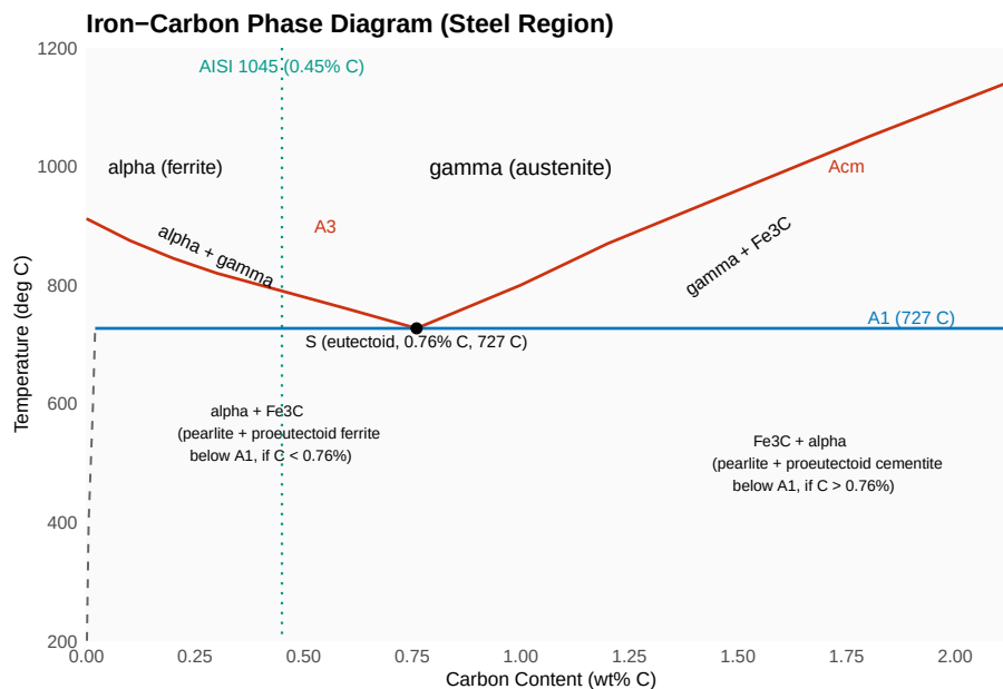
Figure 19.6: The iron-carbon phase diagram, steel region only (0 to 2.14 wt% C). A3 and Acm curves are smoothed approximations for teaching purposes; consult a reference diagram (e.g. Callister) for precise values.
