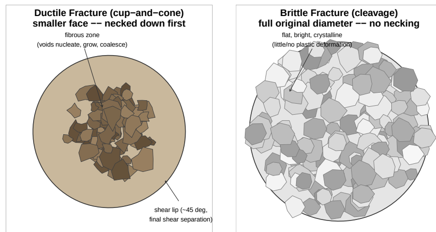
Figure 20.3: Schematic (not photographic) comparison of the two fracture-surface types, drawn at the same scale. Ductile fracture (left) shows a rough, dull, fibrous central zone – where microscopic voids nucleated, grew, and coalesced – ringed by a smoother shear lip at roughly 45 degrees, and the whole face is visibly smaller than the original cross-section because of necking. Brittle fracture (right) shows a flat, bright, crystalline-looking surface with no necking, drawn here at the specimen’s full original diameter for comparison.
