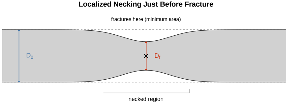
Figure 20.2: Schematic profile of a round tensile specimen showing localized necking (not to scale). Deformation that was uniform along the gauge length concentrates into one local neck once the ultimate tensile strength is passed, and the specimen ultimately fractures at that minimum-diameter cross-section, D_f – the same D_f that Equation 20.4 uses to calculate %RA.
