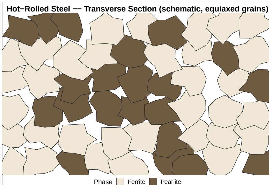
Figure 19.4: Schematic diagram (not an actual photomicrograph) of hot-rolled 1018 steel: equiaxed grains, similar in every direction, regardless of which way the section is cut.
