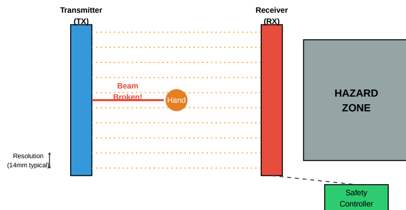
Figure 6.6: Light Curtain Operating Principle
