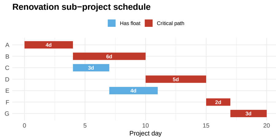
Figure 6.4: The seven-activity renovation network as a Gantt chart. Critical path A-B-D-F-G is dark; C and E (light) carry the float visible as the gap between where they finish and where F can actually start.
