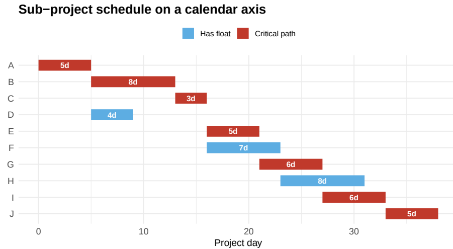
Figure 6.3: The ten-activity sub-project network, redrawn as a Gantt chart from the same ES/EF/float numbers as the float chart above. Dark bars (A, B, C, E, G, I, J) are the critical path; light bars (D, F, H) carry float.
