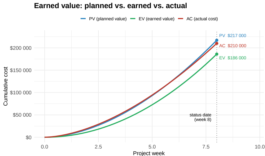
Figure 12.2: The three curves through week 8 of the RC-vehicle project (BAC = $620 000, off the top of this view). By the status date EV sits below PV – behind schedule – and AC sits above EV – over cost. The vertical gaps at week 8 are the schedule and cost variances.
