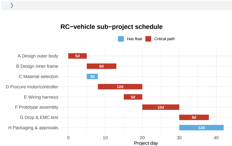
Figure 8.1: A Gantt chart for the RC-vehicle sub-project. Bars are activities; the dark segments show the critical path. Arrows (implied by stacking) show that assembly cannot start until design finishes.
