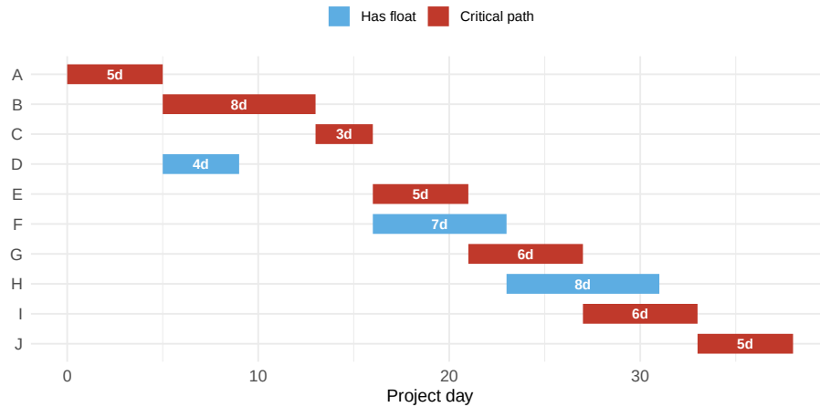
Figure 6.3: The ten-activity sub-project network, redrawn as a Gantt chart from the same ES/EF/float numbers as the float chart above. Dark bars (A, B, C, E, G, I, J) are the critical path; light bars (D, F, H) carry float.
