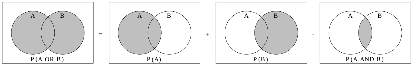
Fig. 3.4.2 A diagram of the addition rule (P(A \text{ OR } B) = P(A) + P(B) - P(A \text{ AND } B)) . Notice event (A \text{ AND } B) , represented by the intersection of the two circles, is counted once when we calculate (P(A)) and again when we calculate (P(B)) . Because we double count this event, we have to subtract (P(A \text{ AND } B)) once to correct for the overcounting.
