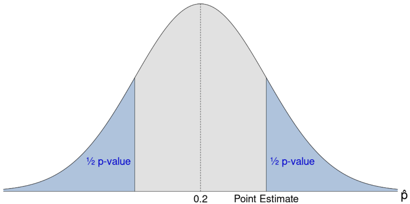
Fig. 6.4.3 The sampling distribution of the population in this example is shown and illustrates a two-tailed test. In a two-tailed test, we first find just half of the \backslash(p\backslash) -value by calculating the probability to the left or right of the point estimate depending on which tail the point estimate is closer to. (In this figure, the point estimate is closer to the right tail, so we would calculate the probability to the right of the point estimate.) Then we double the probability to get the full \backslash(p\backslash) -value. Doubling the probability we initially calculate includes the mirror probability in the opposite tail in the \backslash(p\backslash) -value.
