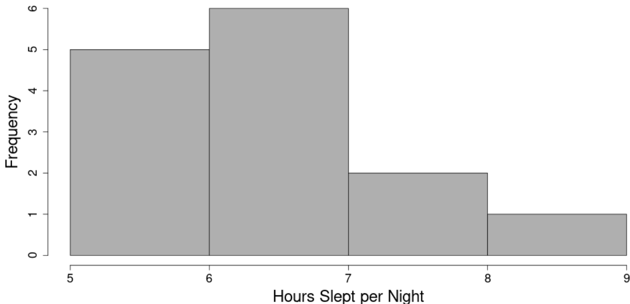
Fig. 1.1.1 A histogram of the data above. The height of each bar in the histogram tells us how many data values we have in the range covered by the histogram. For example, we can see that 5 of the individuals surveyed sleep between 5 and 6 hours per night.
