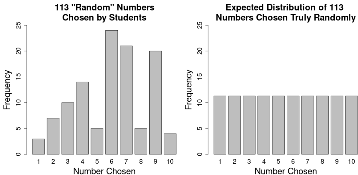
Fig. 1.3.2 The bar chart on the left shows how many times each number from 1 to 10 was chosen by 113 students. The bar chart on the right shows how many times we would expect each number to be chosen if the numbers were actually chosen randomly. The dramatic differences in the bar charts suggest that the students did not truly choose their numbers randomly.
