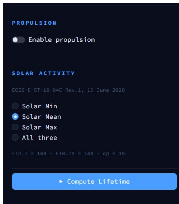
Figure 12: Solar activity. The ECSS Min/Mean/Max scenarios (or all three) set the F10.7 and Ap indices that drive atmospheric density. Solar Mean is shown, with its indices displayed live.
