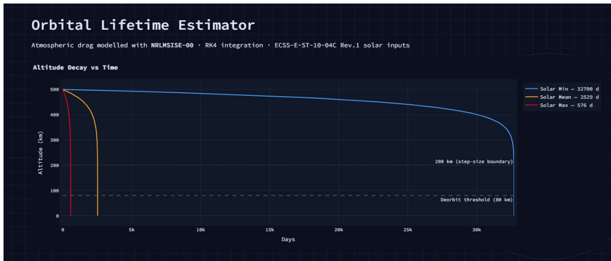
Figure 14: Lifetime decay plot. Altitude versus time for the three solar scenarios overlaid, with the 200 km step-size boundary and the deorbit threshold marked. The order-of-magnitude spread between Solar Max and Min shows the dominant role of solar activity.
