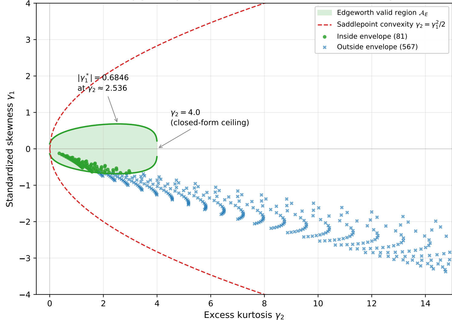
Admissibility geometry: Edgeworth envelope and 648-cell rare-disaster grid
