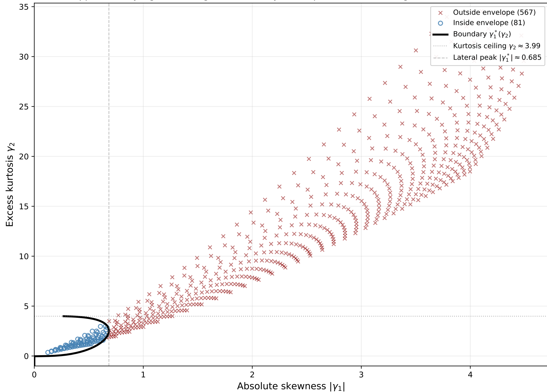
Supplementary Figure S1. Edgeworth validity envelope — rare-disaster grid (648 combinations)
