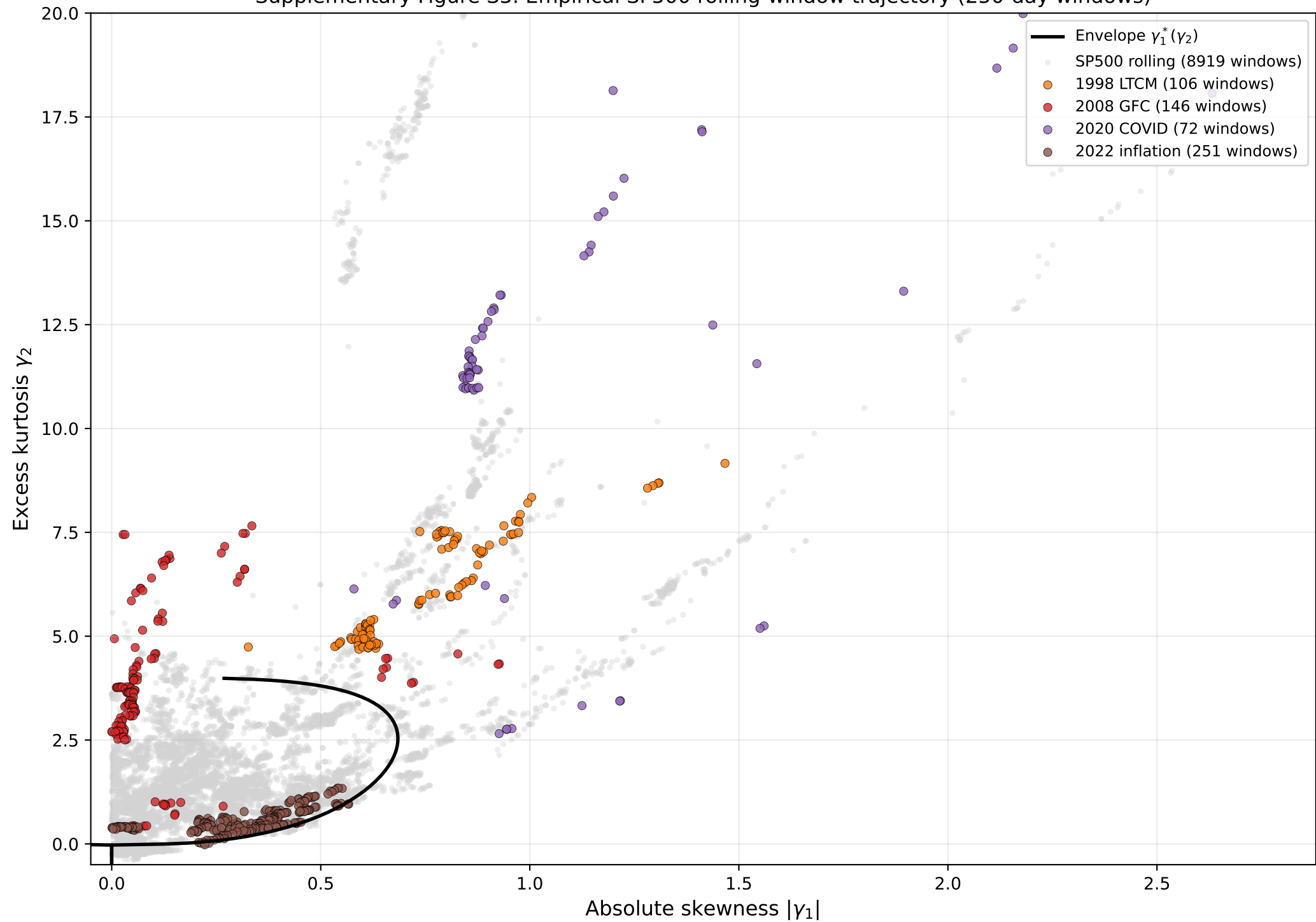
Supplementary Figure S3. Empirical SP500 rolling-window trajectory (250-day windows)
