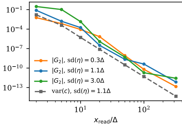
(b) dependence on readout field
