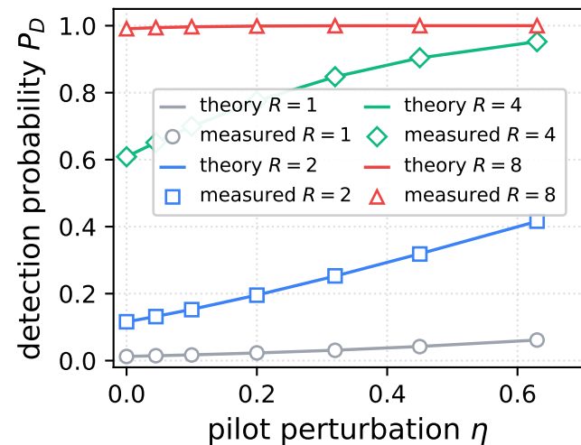
(a) P_D vs \eta ( P_{FA} = 10^{-6} , BT = 10^6 )
