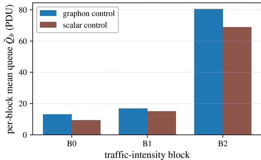
Per-region QoS disparity ( 6.1\times )
