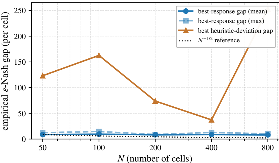
Best-response \varepsilon -Nash gap on milan topology
