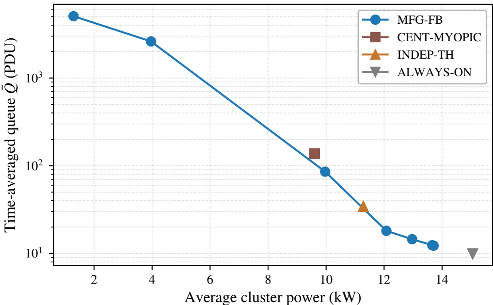
Energy/queue Pareto sweep over c_p/c_q ( N=100 )
